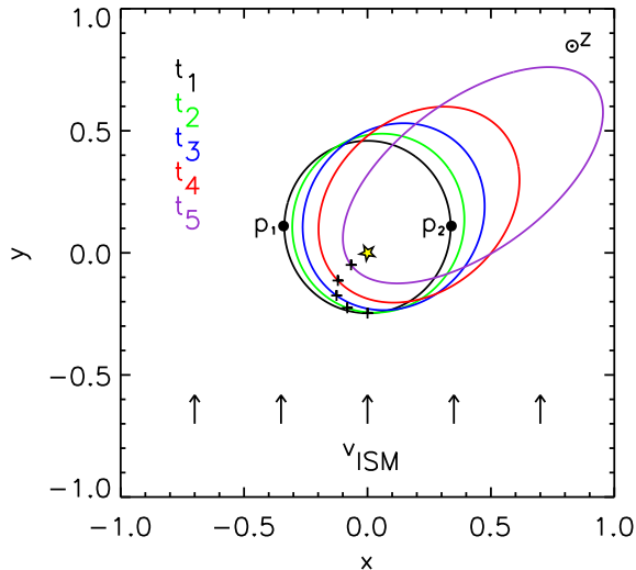
FIG. 10.— Orbital evolution of a test particle in the x-y plane under the effect of neutral gas drag. Five time periods separated by a fixed number of orbits are shown. The grain begins with its star-pericenter (Runge-Lenz) vector anti-aligned with the incoming interstellar flow, directed along the positive y -axis, and its angular momentum vector aligned with the z -axis (out of the page). The ISM flow decelerates the grain on one leg (e.g., point p_1 ) and accelerates it on the other (e.g., point p_2 ), causing the Runge-Lenz vector to rotate. The grain’s periastron at each successive time is shown by a cross to illustrate this effect.
