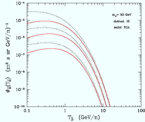
FIG. 4: Antideuteron flux for WIMPs of m_{\chi}=50 GeV. Dotted (black) lines refer to the interstellar flux, solid (red) lines stand for the top-of-atmosphere flux, modulated at solar minimum. For each set of curves, the three lines refer to the maximal, median and minimal propagation configurations defined in Table I.
