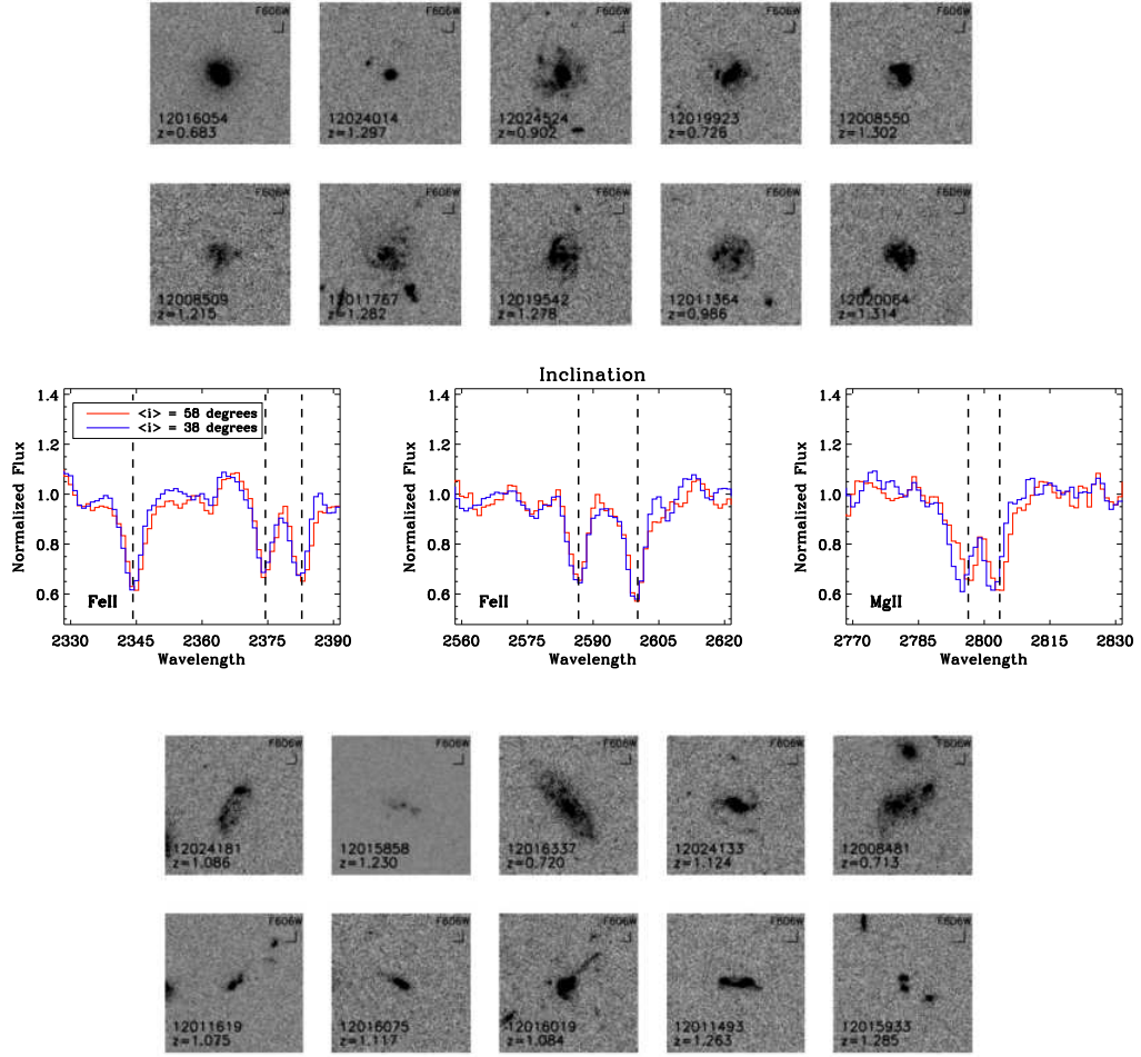
Figure 3.21 Composite spectra assembled from objects with high and low inclinations, respectively, where inclinations were estimated from HST V + I band imaging assuming intrinsic circular disks: i = \cos^{-1}[b/a] (Tully & Fisher, 1977). We find that the composite spectrum composed of high inclination objects (red line) is best-fit with V_1 = 28 \pm 11 \text{ km s}^{-1} while the composite spectrum assembled from low inclination galaxies (blue line) has a V_1 outflow velocity of -19 \pm 9 \text{ km s}^{-1} . Even though the overall shifts of each composite from 0 \text{ km s}^{-1} are small in magnitude, the kinematic difference between the two composites is significant. These results are consistent with the trend of stronger blueshifts with decreasing inclination, as noted by Chen et al. (2010) for a local sample of SDSS galaxies. V -band thumbnails of the ten lowest and highest inclination objects are shown above and below the composite spectra, respectively.
