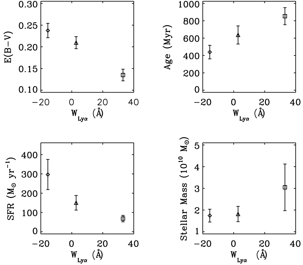
Figure 2.8 Best-fit stellar population parameters versus rest-frame \text{Ly}\alpha equivalent width. Omitting galaxies with K_s upper limits, the remaining 179 objects with stellar population modeling were ordered by equivalent width and divided into three groups. The average stellar population parameters of each group were extracted, along with the error on the mean ( \sigma/\sqrt{n} , where n was the number of objects in each group). With increasing \text{Ly}\alpha strength, galaxies are, on average, older, less dusty, and more quiescent. A weak trend of increasing stellar mass with increasing \text{Ly}\alpha strength is observed, although this is likely not a significant correlation.
