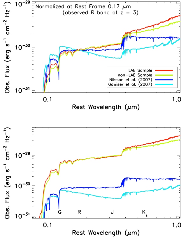
Figure 2.10 Top panel: Composite rest-frame UV to near-infrared SEDs of the LAE and non-LAE samples, assembled from best-fit SEDs from population synthesis modeling (omitting galaxies with K_s upper limits). Data from z \sim 3.1 narrowband-selected LAEs (Nilsson et al., 2007; Gawiser et al., 2007) are overplotted and all spectra have been normalized to the Nilsson et al. (2007) flux value at 0.17 \mu\text{m} (observed \mathcal{R} band at z \sim 3 ). Note that the LBG-selected objects have significantly redder G - \mathcal{R} and \mathcal{R} - K_s colors than the narrowband-selected LAEs, consistent with the older ages and higher dust attenuations derived for LBGs in the literature. Bottom panel: Un-normalized spectra; note the significant flux discrepancy ( \sim 2.3 magnitudes) between the color-selected LBGs and the narrowband-selected LAEs.
