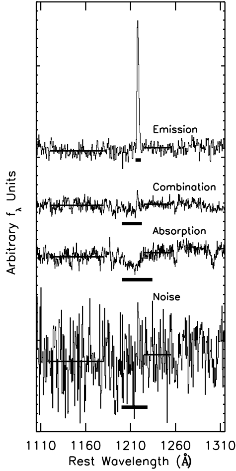
Figure 2.2 The \text{Ly}\alpha feature varies widely in its morphology. Four spectra are plotted to show representative examples of objects classified in the “emission,” “combination,” “absorption,” and “noise” bins, respectively. In order to systematically calculate \text{Ly}\alpha equivalent width, we adopted red- and blue-side continua (horizontal lines from 1120–1180 Å and from 1225–1255 Å, respectively) and inferred the extent of the \text{Ly}\alpha feature (thick line below each spectrum) using the methodology described in §2.1.3. Note that in the case of the “absorption” spectrum shown here, the extent of the \text{Ly}\alpha feature appears to extend redwards of the adopted red-side continuum – this difference arises because the plotted spectrum is unsmoothed while a smoothed spectrum was employed to calculate the wavelength bounds of the \text{Ly}\alpha feature.
